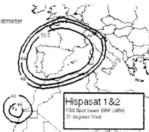
Fig.1: HISPASAT 1 and 2 Footprints
