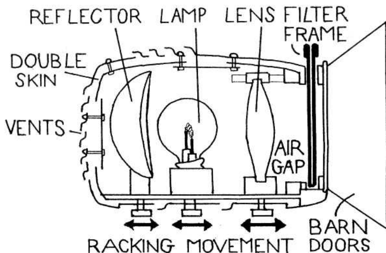
Fig.1: Composite Features of a Lantern
