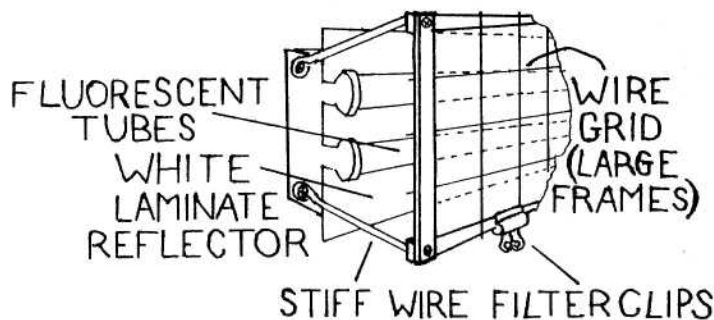
Fig.2: Construction of Softlight source
