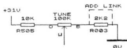
Fig.1 and Fig.2: Extending the Tuning Range
